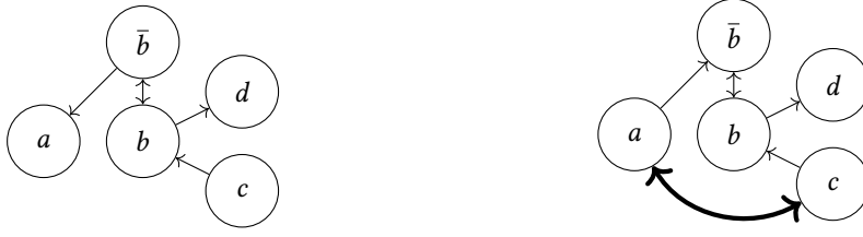
Figure 3: Two abstract AF representations where a is sufficient support for b , providing closure under supported and mediated attacks. In the right graph, since a \in \bar{b} we must have a \in c^- \cup c^+ .
